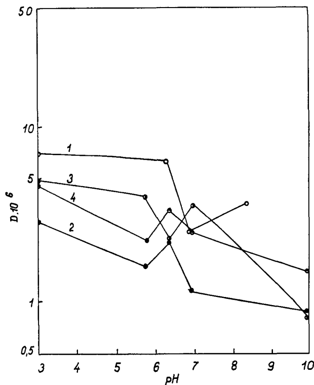
Figure 1. Self-diffusion coefficients of ^{106}\text{Ru} , ^{144}\text{Ce} , ^{147}\text{Pm} , and ^{156}\text{Eu} vs. \text{pH} . 94,95 Ionic strength \mu = 0.01 ( \text{NaCl} ); D = self-diffusion coefficient, \text{cm}^2/\text{sec} ; curve 1 for ^{106}\text{Ru} , curve 2 for ^{144}\text{Ce} , curve 3 for ^{147}\text{Pm} , curve 4 for ^{156}\text{Eu} .
